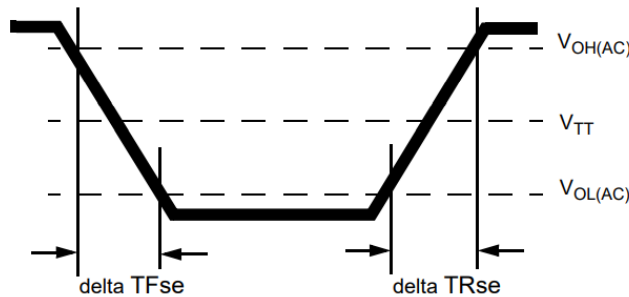
Figure 17. Single-ended Output Slew Rate Definition
