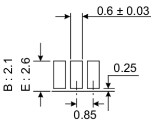
Detail B,E
