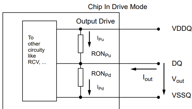
Figure 15. Output driver
