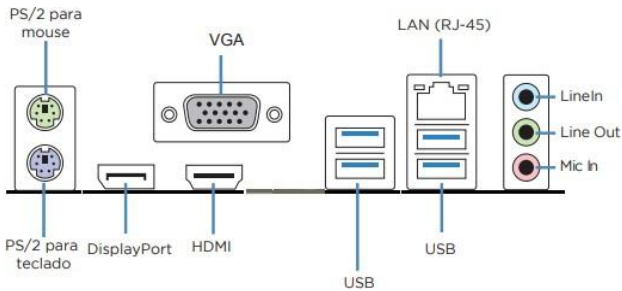
Painel Traseiro
