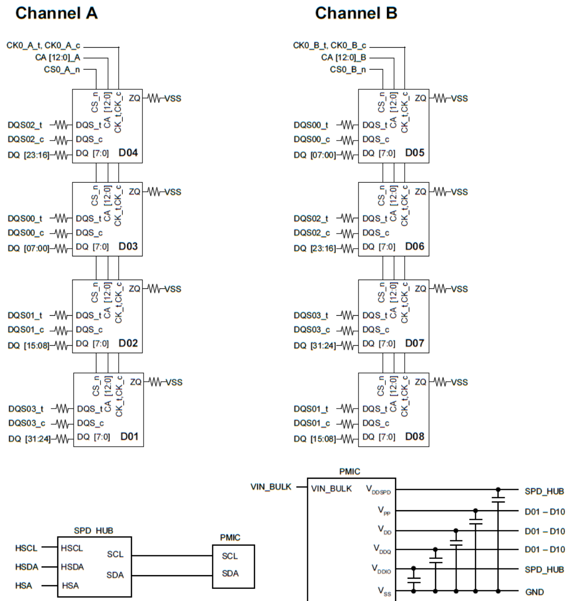
Figure 4-1 1Rank, x8 DDR5 SDRAMs
