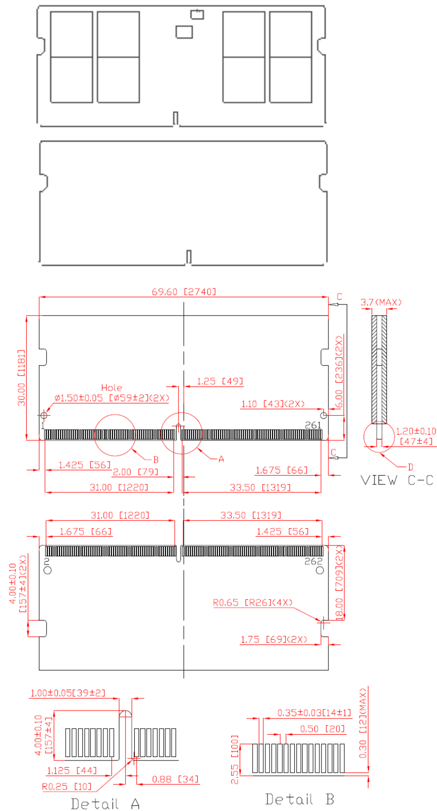
Figure 12-1 Physical Dimensions
